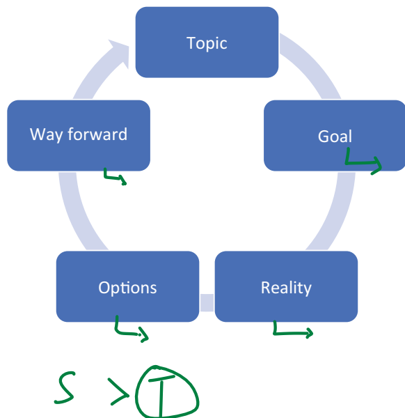
Fig. 15.1 GROW Model
