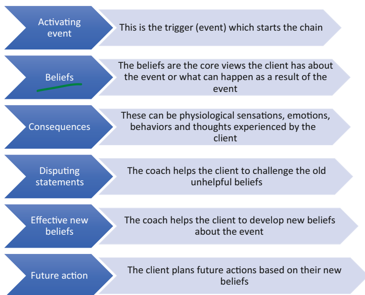
Fig. 17.1 ABCDEF Model
